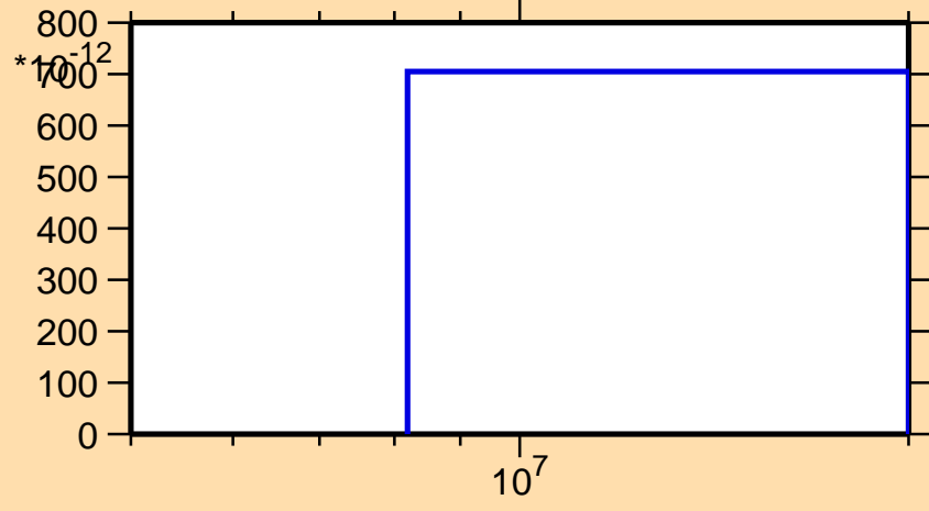
\sigma vs. E for ^{188}\text{Hg} (mt 45)
