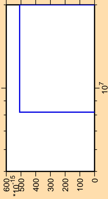
\Delta\sigma/\sigma vs. E for ^{188}\text{Hg} (mt 11)
