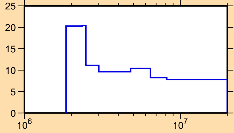
\Delta\sigma/\sigma vs. E for ^{188}\text{Hg}(n,n\text{onel.})
