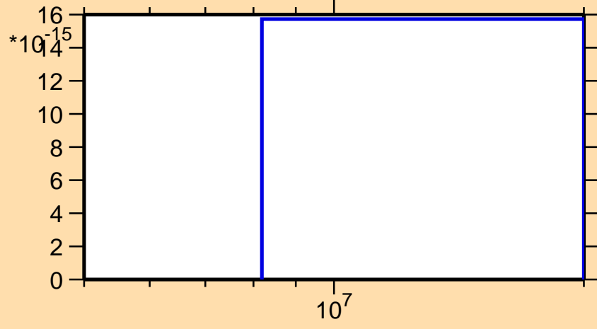
\sigma vs. E for ^{188}\text{Hg} (mt 34)
