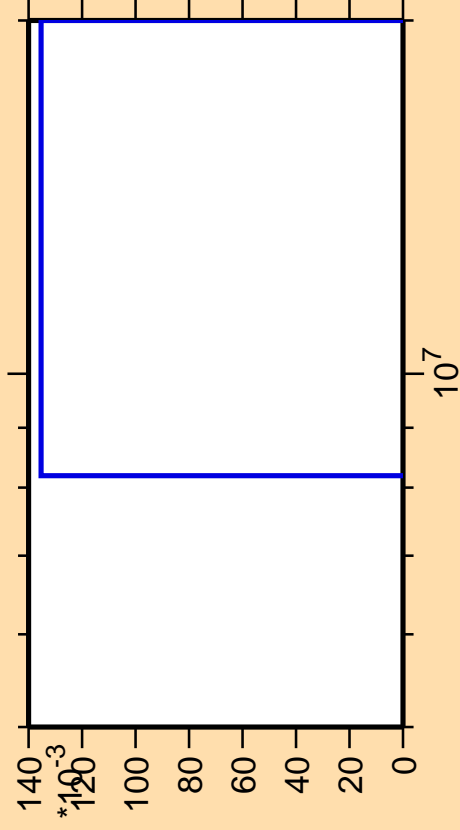
\Delta\sigma/\sigma vs. E for ^{188}\text{Hg} (mt 34)
