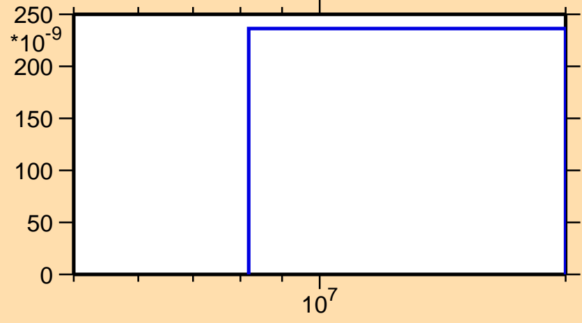
\sigma vs. E for ^{188}\text{Hg}(n,2n\alpha)
