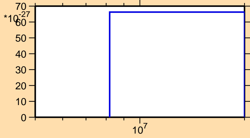
\sigma vs. E for ^{188}\text{Hg} (mt 11)
