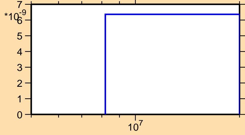
\sigma vs. E for ^{188}\text{Hg}(n,2np)
