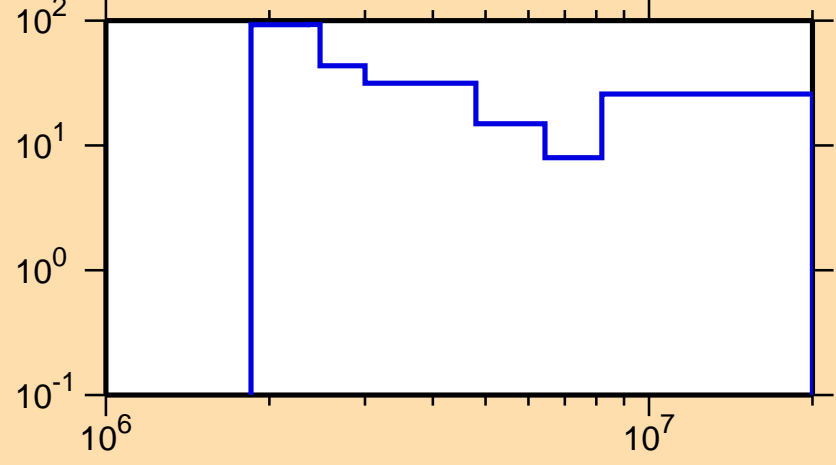
\Delta\sigma/\sigma vs. E for ^{188}\text{Hg}(n,\text{inel.})
