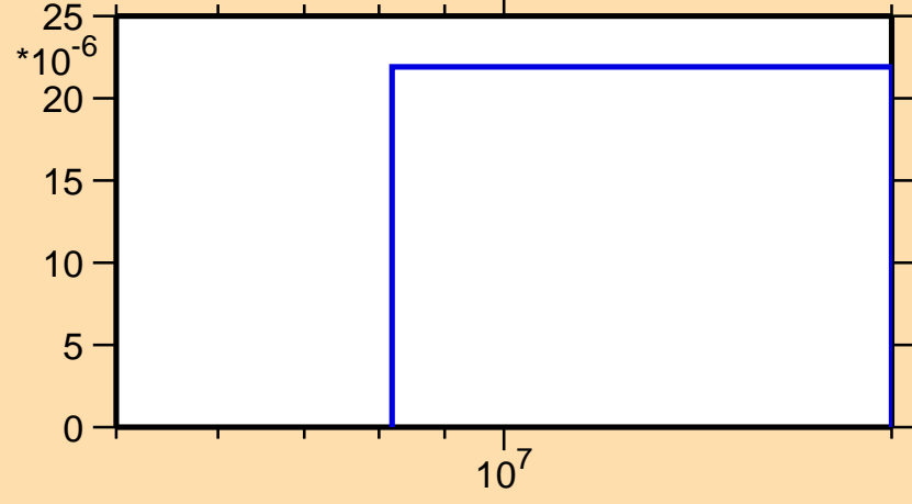
\sigma vs. E for ^{188}\text{Hg}(n,t)
