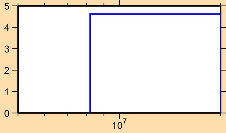
\Delta\sigma/\sigma vs. E for ^{188}\text{Hg}(n,\text{el.})
