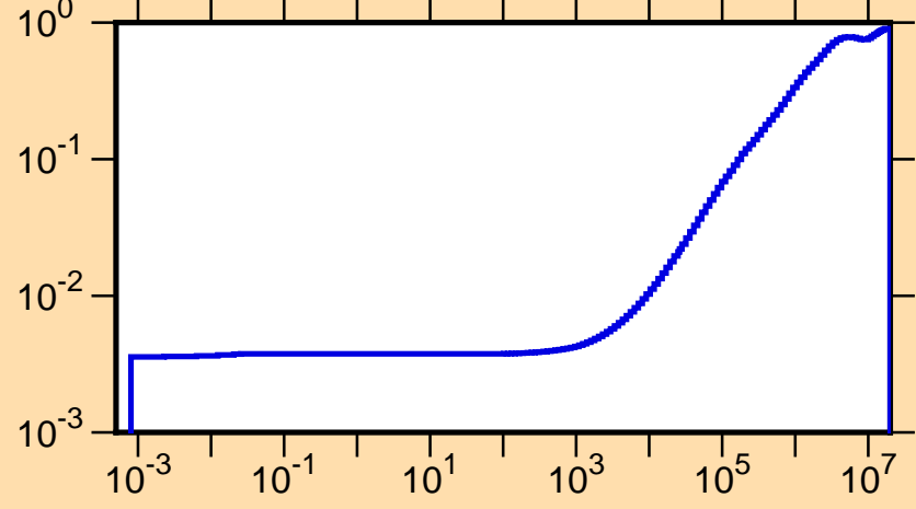
\mu vs. E for ^{189}\text{Hg}(\text{mt251})
