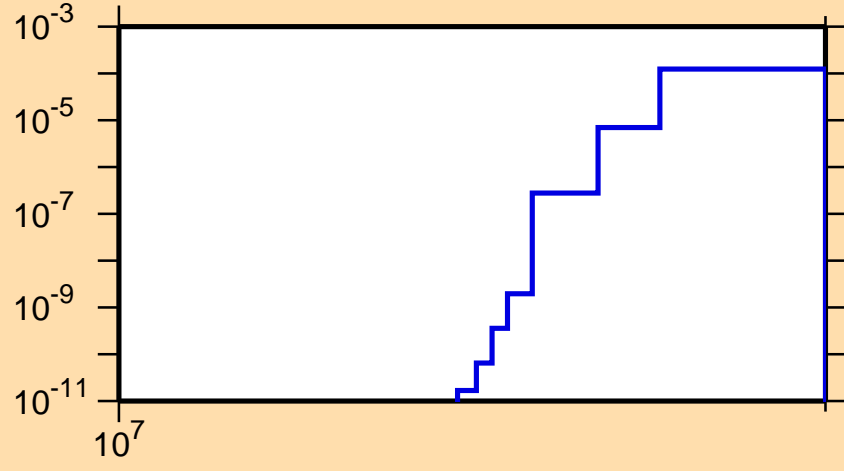
\sigma vs. E for ^{189}\text{Hg}(n,2np)
