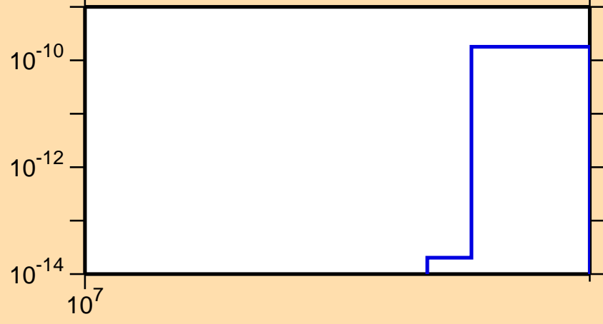
\sigma vs. E for ^{189}\text{Hg}(n,\text{nt})
