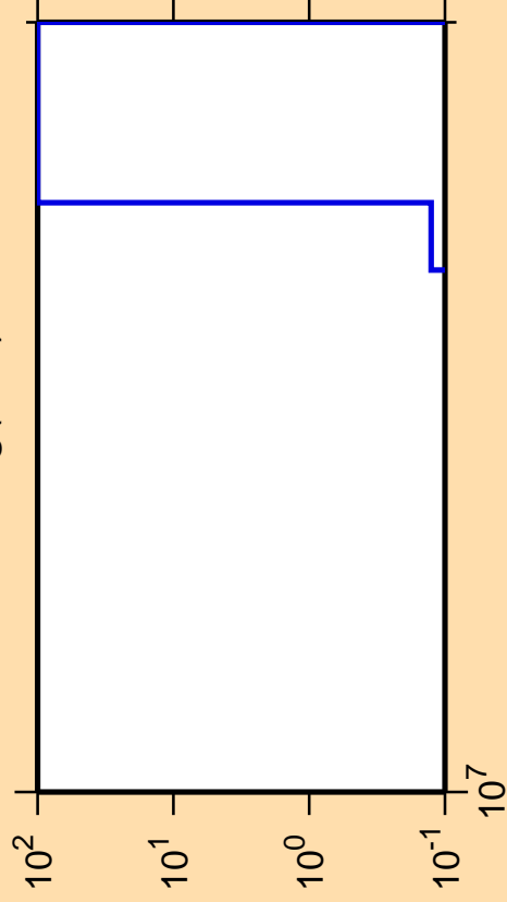
\Delta\sigma/\sigma vs. E for ^{189}\text{Hg}(n,\text{nt})
