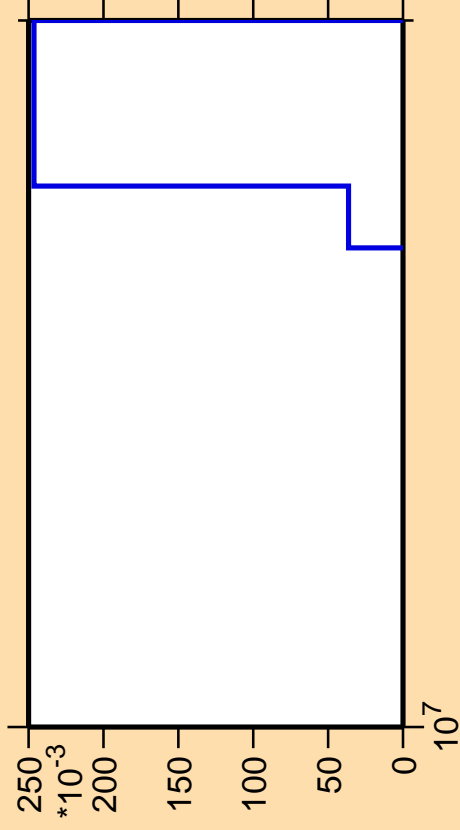
\Delta\sigma/\sigma vs. E for ^{189}\text{Hg}(n,3n\alpha)
