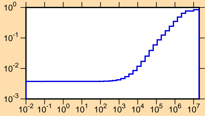
\mu vs. E for ^{189}\text{Hg}(\text{mt251})
