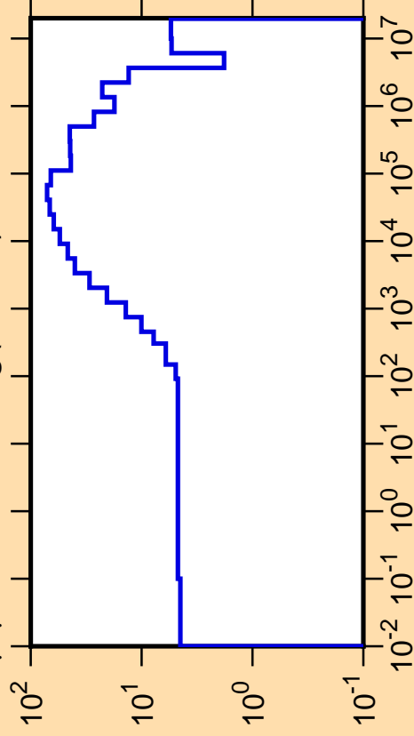
\Delta\mu/\mu vs. E for ^{189}\text{Hg}(\text{mt251})
