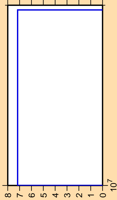
\Delta\sigma/\sigma vs. E for ^{189}\text{Hg}(n,\text{nt})
