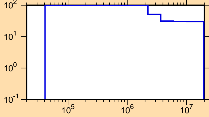
\Delta\sigma/\sigma vs. E for ^{189}\text{Hg}(n,n_1)
