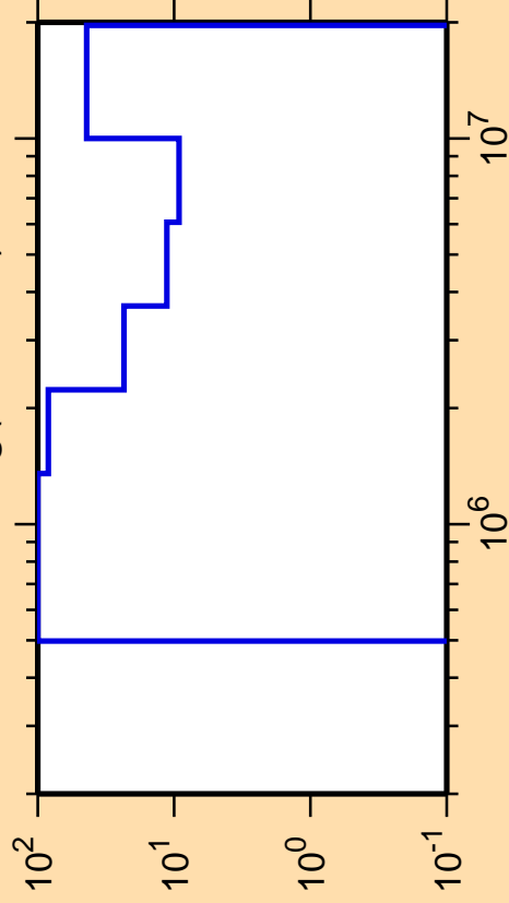
\Delta\sigma/\sigma vs. E for ^{189}\text{Hg}(n,\text{ncont.})
