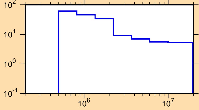
\Delta\sigma/\sigma vs. E for ^{189}\text{Hg}(n,n\text{onel.})
