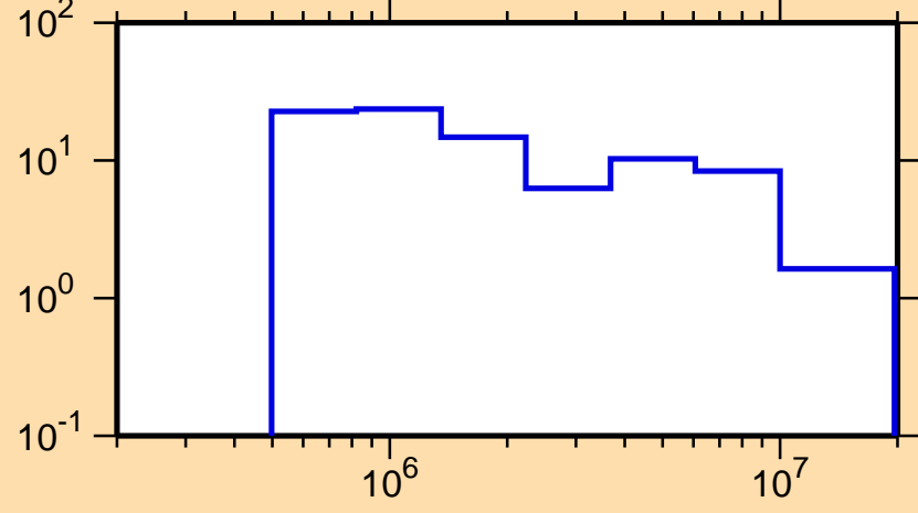
\Delta\sigma/\sigma vs. E for ^{189}\text{Hg}(n,\text{tot.})
