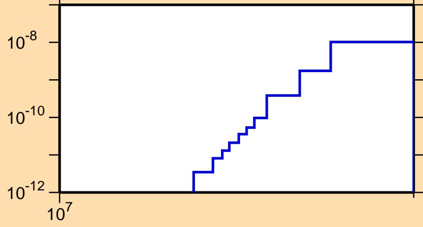
\sigma vs. E for ^{189}\text{Hg} (mt 45)
