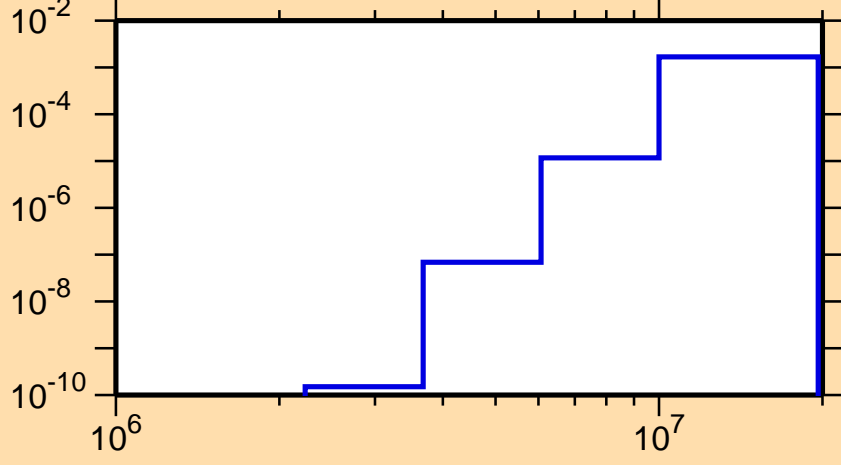
\sigma vs. E for ^{189}\text{Hg}(n,n\alpha)
