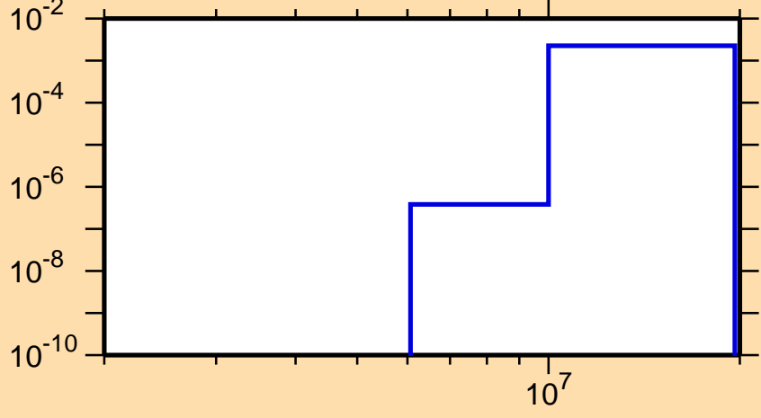
\sigma vs. E for ^{189}\text{Hg}(n,d)
