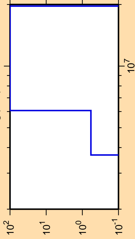
\Delta\sigma/\sigma vs. E for ^{189}\text{Hg}(n,d)
