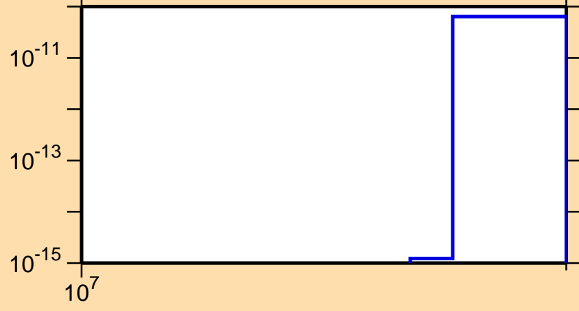
\sigma vs. E for ^{190}\text{Hg}(n,nt)
