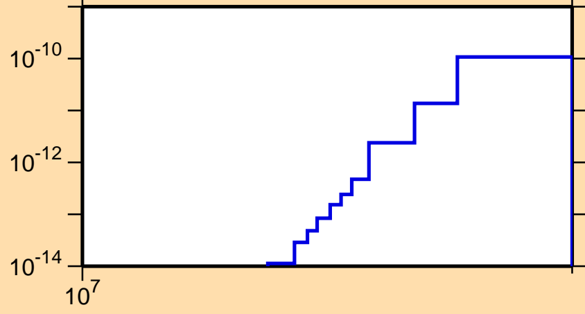
\sigma vs. E for ^{190}\text{Hg}(\text{mt117})
