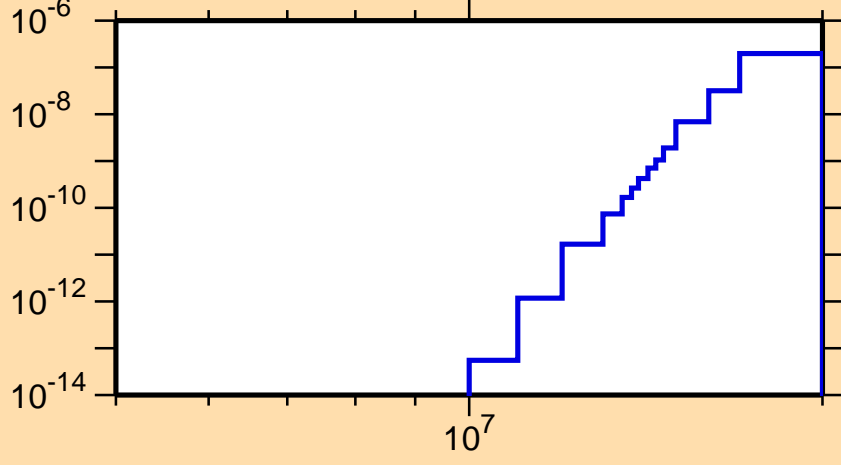
\sigma vs. E for ^{190}\text{Hg}(n,\text{He}3)
