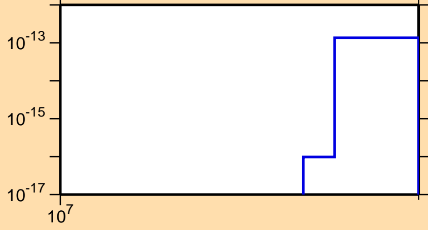
\sigma vs. E for ^{190}\text{Hg}(n,\text{pt})
