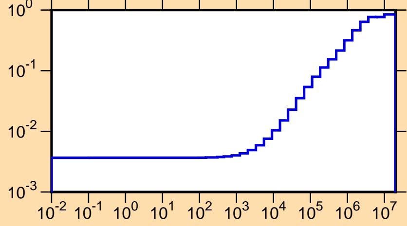
\mu vs. E for ^{190}\text{Hg}(\text{mt251})
