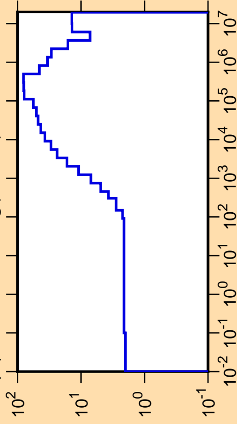
\Delta\mu/\mu vs. E for ^{190}\text{Hg}(\text{mt251})
