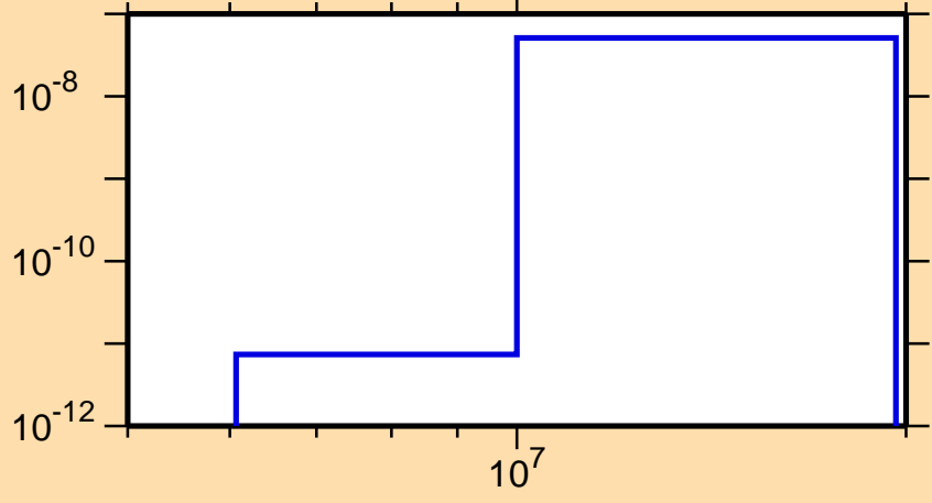
\sigma vs. E for ^{190}\text{Hg}(n,p\alpha)
