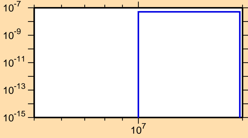
\sigma vs. E for ^{190}\text{Hg}(n,2n\alpha)
