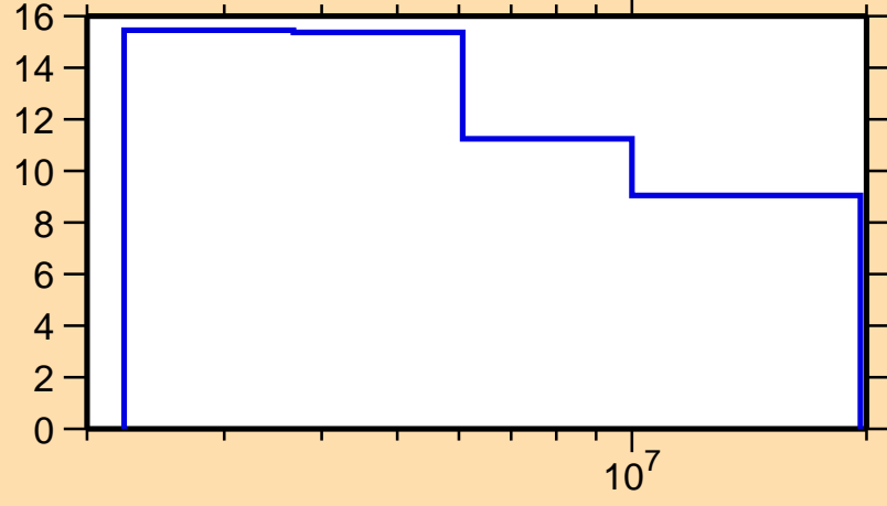
\Delta\sigma/\sigma vs. E for ^{190}\text{Hg}(n,n\text{onel.})
