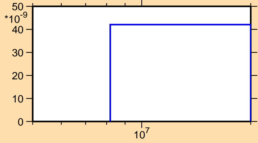
\sigma vs. E for ^{190}\text{Hg}(n,2n\alpha)
