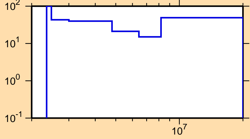
\Delta\sigma/\sigma vs. E for ^{190}\text{Hg}(n,n\text{cont.})
