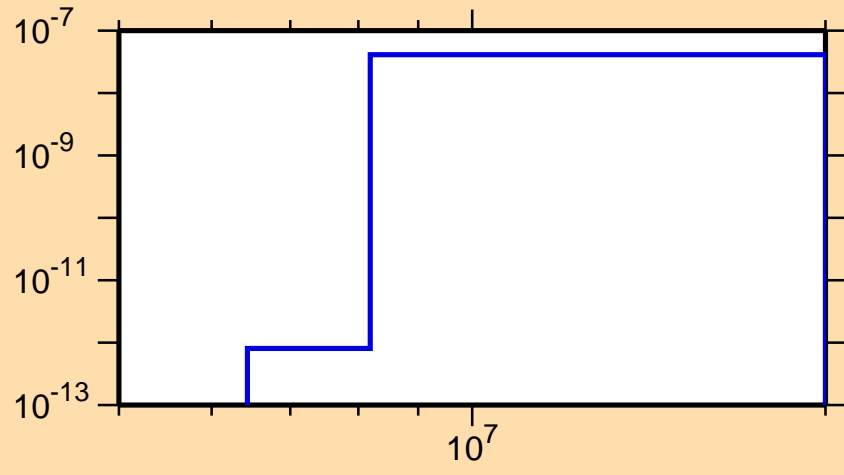
\sigma vs. E for ^{190}\text{Hg}(n,p\alpha)
