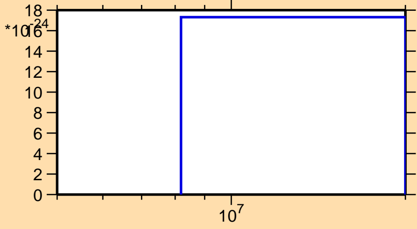
\sigma vs. E for ^{190}\text{Hg} (mt 11)
