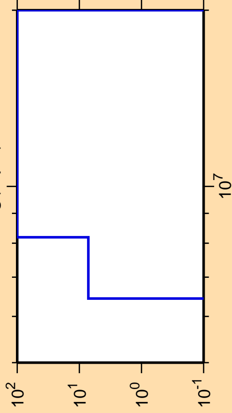
\Delta\sigma/\sigma vs. E for ^{190}\text{Hg}(n,p\alpha)
