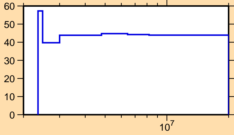
\Delta\sigma/\sigma vs. E for ^{190}\text{Hg}(n,n_1)
