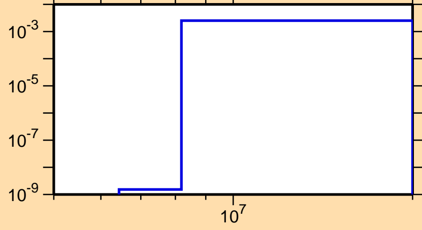
\sigma vs. E for ^{190}\text{Hg}(n,np)
