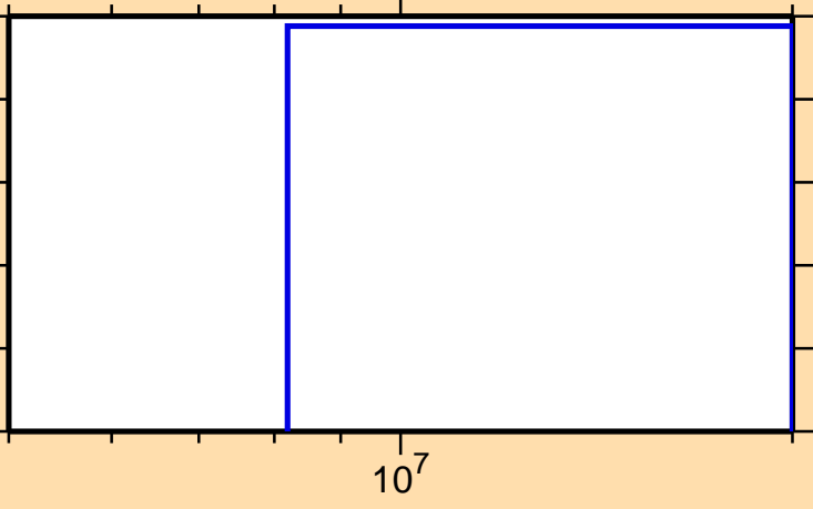
\sigma vs. E for ^{190}\text{Hg}(n,2np)
