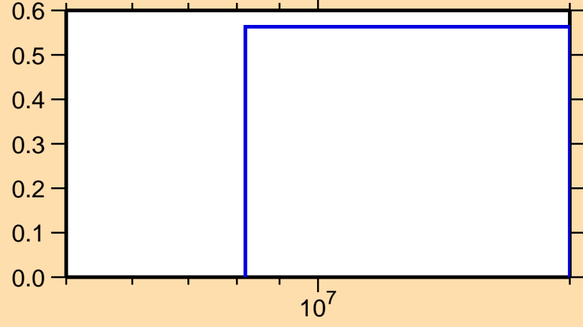
\sigma vs. E for ^{190}\text{Hg}(n,2n)
