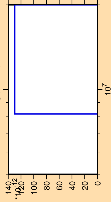
\Delta\sigma/\sigma vs. E for ^{190}\text{Hg} (mt 11)
