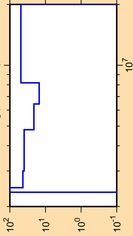
\Delta\sigma/\sigma vs. E for ^{190}\text{Hg}(n,\text{ncont.})
