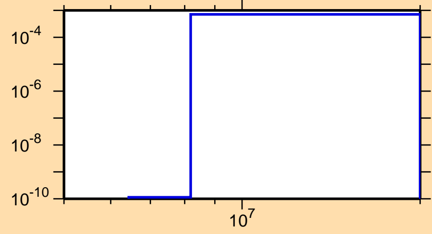
\sigma vs. E for ^{190}\text{Hg}(n,d)
