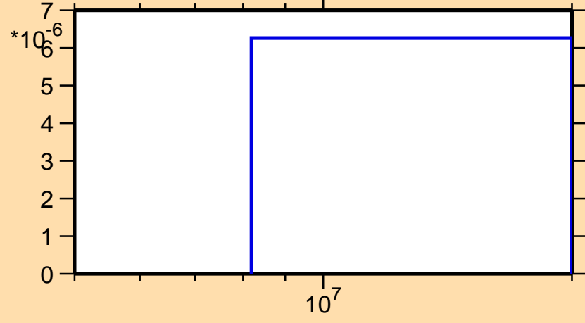
\sigma vs. E for ^{190}\text{Hg}(n,3n)
