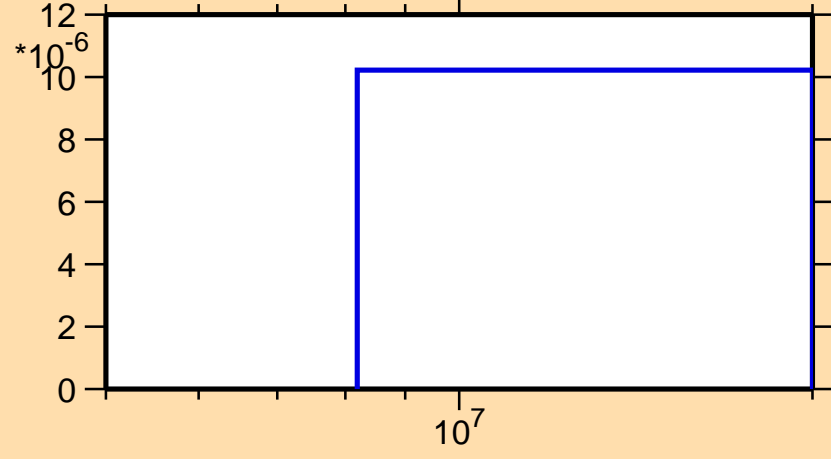
\sigma vs. E for ^{190}\text{Hg}(n,t)
