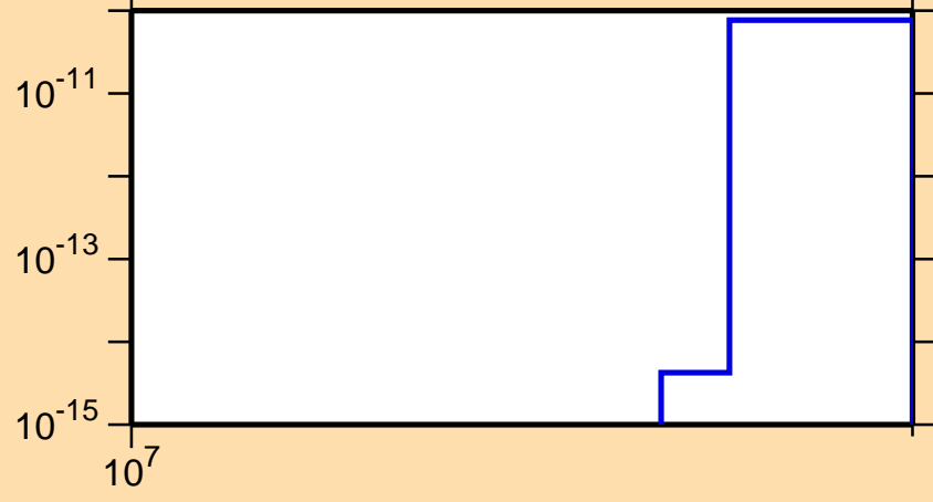
\sigma vs. E for ^{191}\text{Hg}(n,nt)
