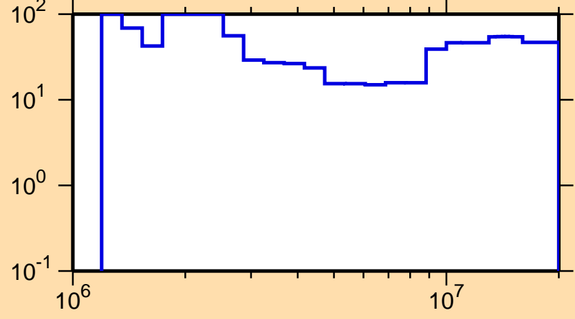
\Delta\sigma/\sigma vs. E for ^{191}\text{Hg}(n,n\text{cont.})
