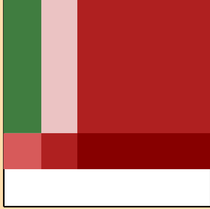
\Delta\sigma/\sigma vs. E for ^{191}\text{Hg}(n,\text{tot.})
