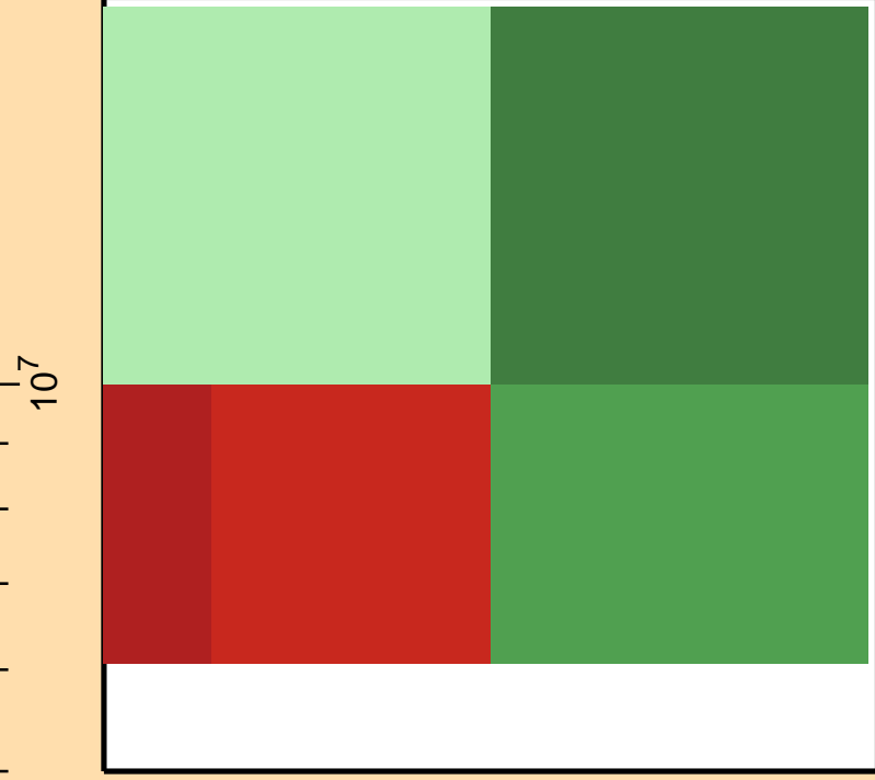
\Delta\sigma/\sigma vs. E for ^{191}\text{Hg}(n,\text{tot.})
