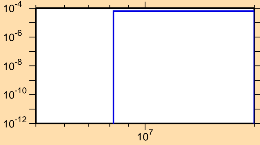
\sigma vs. E for ^{191}\text{Hg}(n,t)
