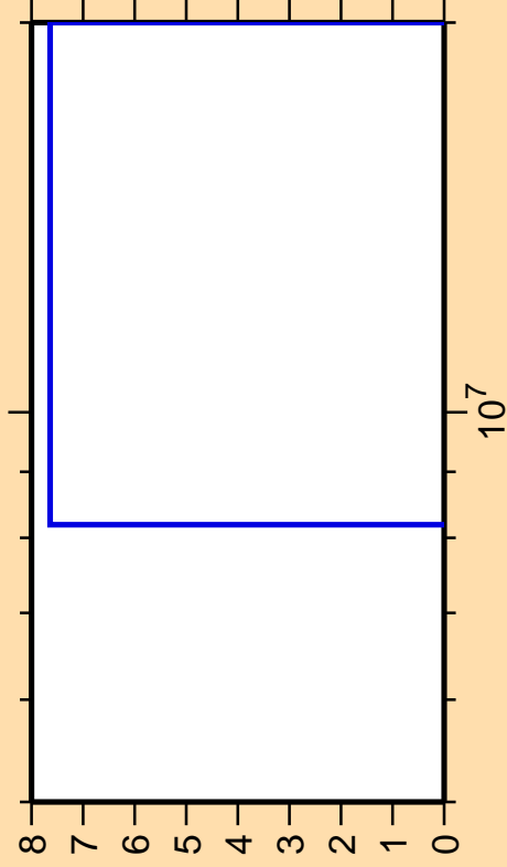
\Delta\sigma/\sigma vs. E for ^{191}\text{Hg} (mt 45)
