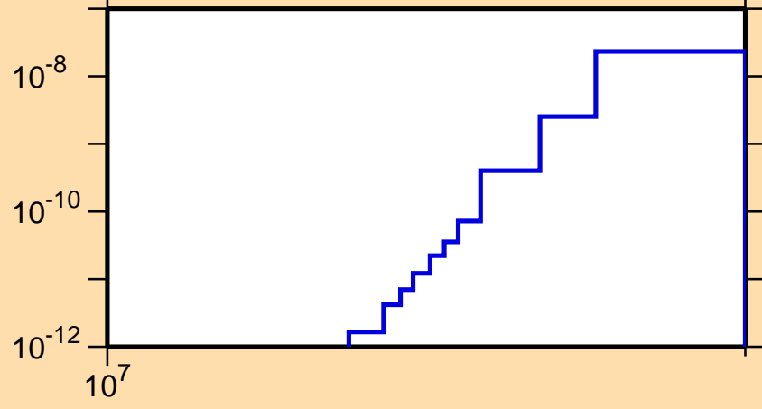
\sigma vs. E for ^{192}\text{Hg}(n,\text{He3})
