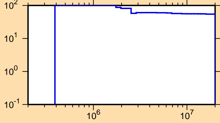
\Delta\sigma/\sigma vs. E for ^{192}\text{Hg}(n,n_1)
