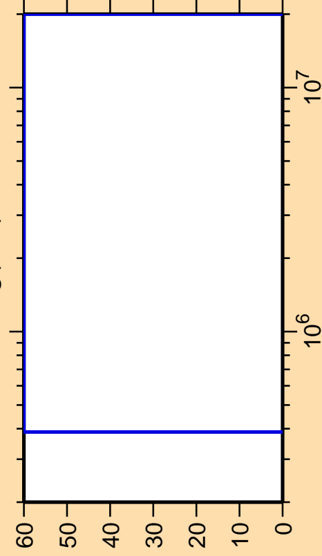
\Delta\sigma/\sigma vs. E for ^{192}\text{Hg}(n,\alpha)
