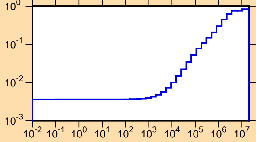
\mu vs. E for ^{192}\text{Hg}(\text{mt251})
