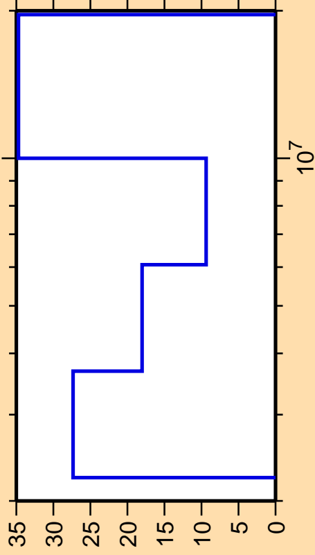
\Delta\sigma/\sigma vs. E for ^{192}\text{Hg}(n,\text{ncont.})
