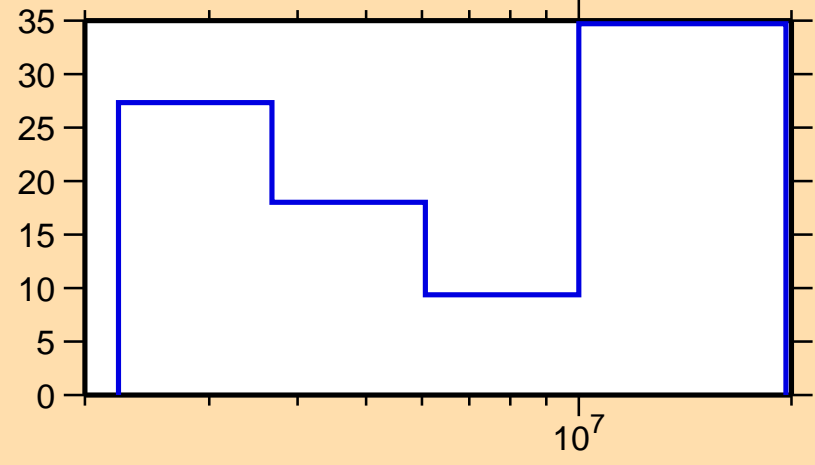
\Delta\sigma/\sigma vs. E for ^{192}\text{Hg}(n,ncont.)
