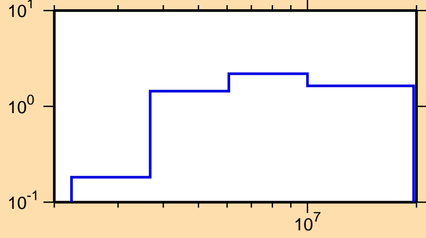
\sigma vs. E for ^{192}\text{Hg}(n,n\text{cont.})
