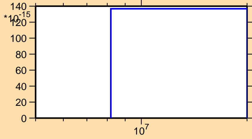
\sigma vs. E for ^{192}\text{Hg}(\text{mt } 45)
