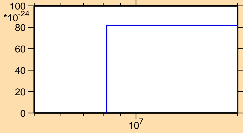
\sigma vs. E for ^{192}\text{Hg}(\text{mt } 11)
