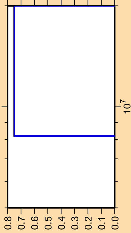
\Delta\sigma/\sigma vs. E for ^{192}\text{Hg}(\text{mt } 45)
