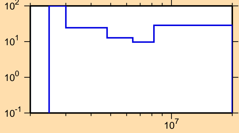
\Delta\sigma/\sigma vs. E for ^{192}\text{Hg}(n,ncont.)
