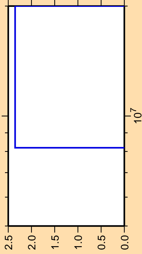
\Delta\sigma/\sigma vs. E for ^{192}\text{Hg}(n,\text{nt})
