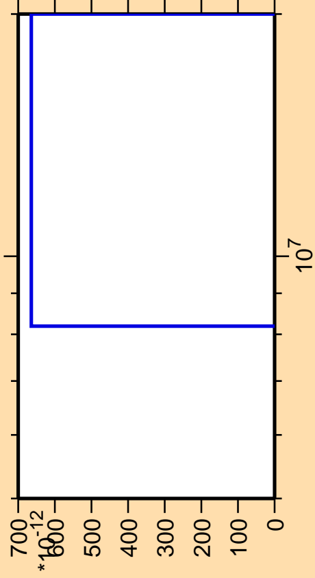
\Delta\sigma/\sigma vs. E for ^{192}\text{Hg}(\text{mt } 11)
