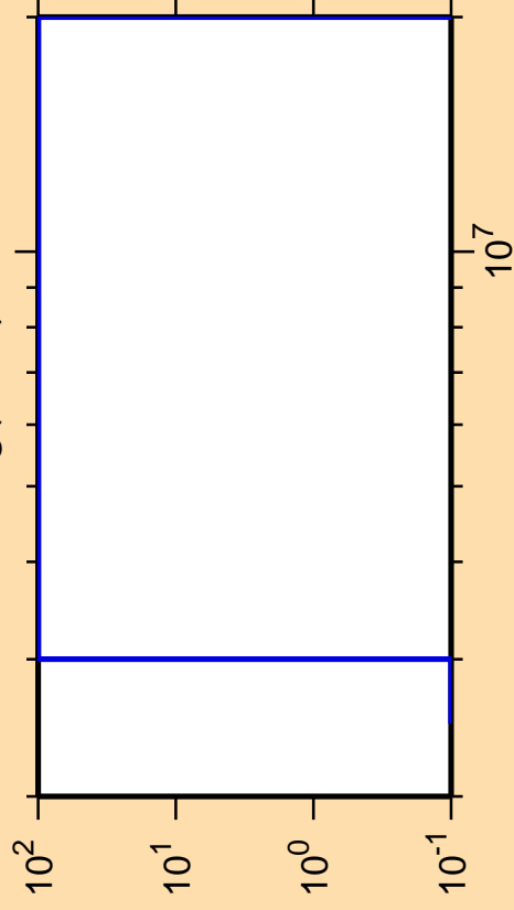
\Delta\sigma/\sigma vs. E for ^{192}\text{Hg}(n,n\alpha)
