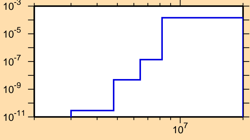
\sigma vs. E for ^{192}\text{Hg}(n,n\alpha)
