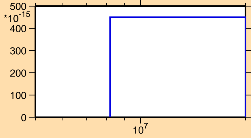
\sigma vs. E for ^{192}\text{Hg}(n,\text{nt})
