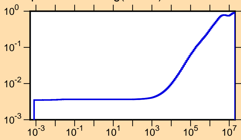
\mu vs. E for ^{193}\text{Hg}(\text{mt251})
