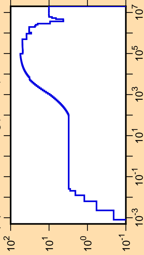
\Delta\mu/\mu vs. E for ^{193}\text{Hg}(\text{mt251})
