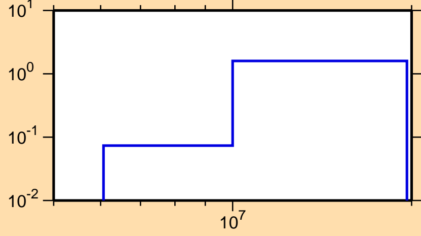
\sigma vs. E for ^{193}\text{Hg}(n,2n)
