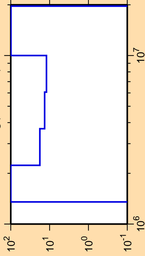
\Delta\sigma/\sigma vs. E for ^{193}\text{Hg}(n,\text{ncont.})
