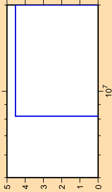
\Delta\sigma/\sigma vs. E for ^{193}\text{Hg}(n,\text{nt})
