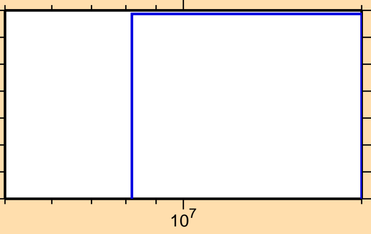
\sigma vs. E for ^{193}\text{Hg}(n,\text{He}3)
