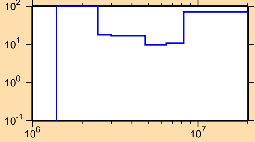
\Delta\sigma/\sigma vs. E for ^{193}\text{Hg}(n,ncont.)
