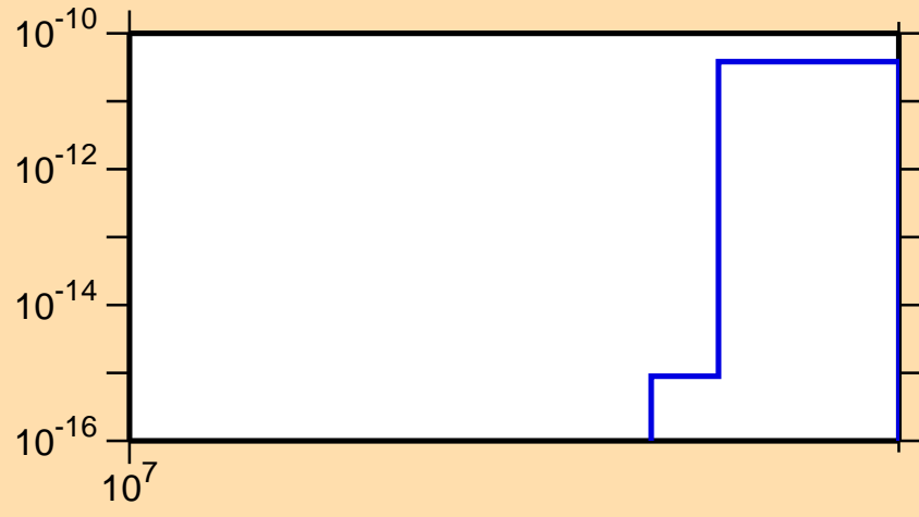
\sigma vs. E for ^{193}\text{Hg}(n,\text{nt})
