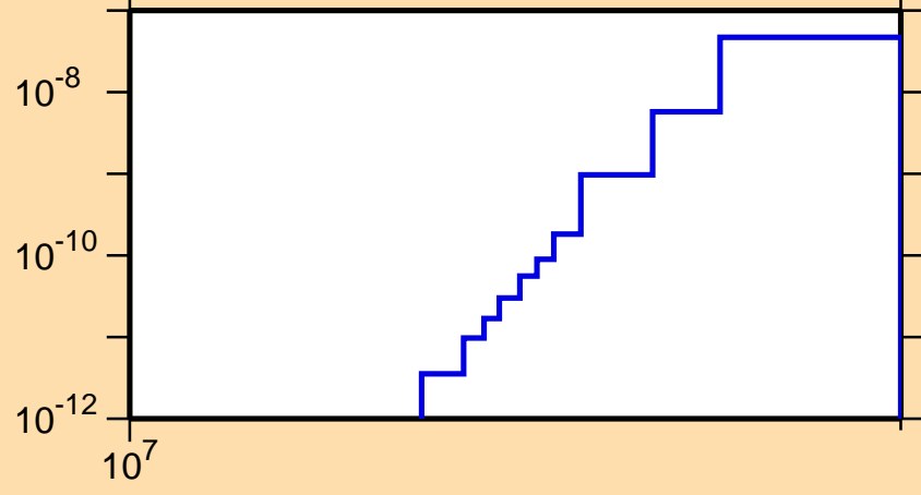
\sigma vs. E for ^{193}\text{Hg}(n,\text{He}3)
