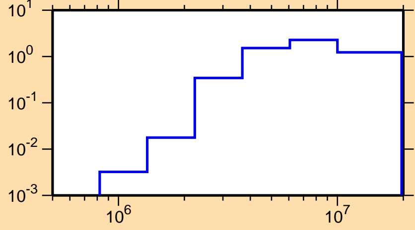
\sigma vs. E for ^{193}\text{Hg}(n,n\text{cont.})
