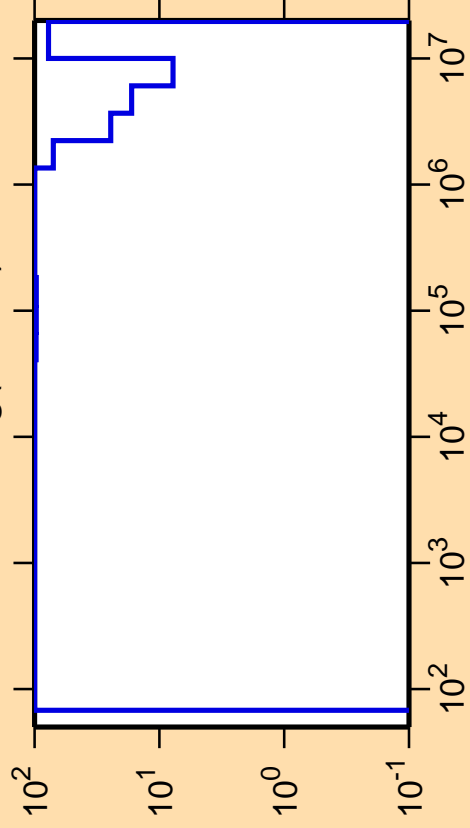
\Delta\sigma/\sigma vs. E for ^{193}\text{Hg}(n,\text{inel.})
