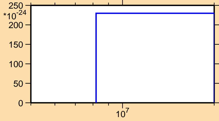
\sigma vs. E for ^{193}\text{Hg}(\text{mt } 11)
