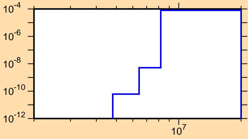
\sigma vs. E for ^{193}\text{Hg}(n,n\alpha)
