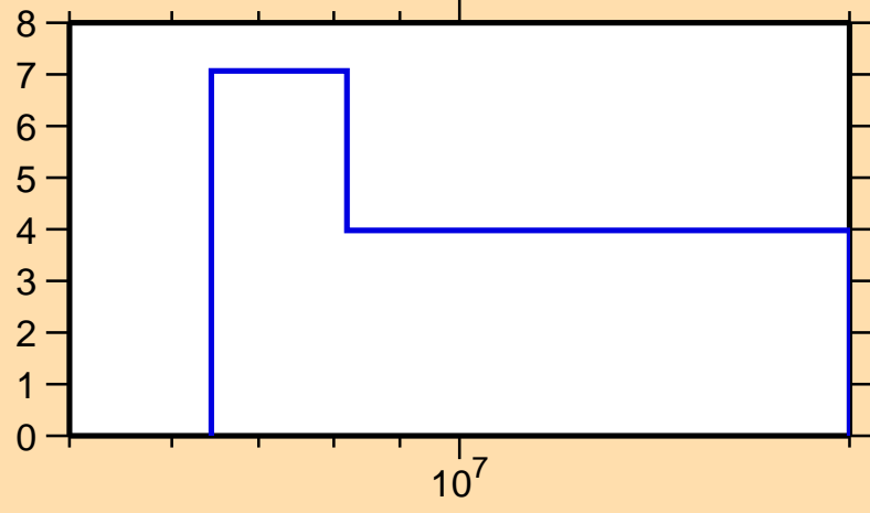
\Delta\sigma/\sigma vs. E for ^{193}\text{Hg}(n,\text{tot.})
