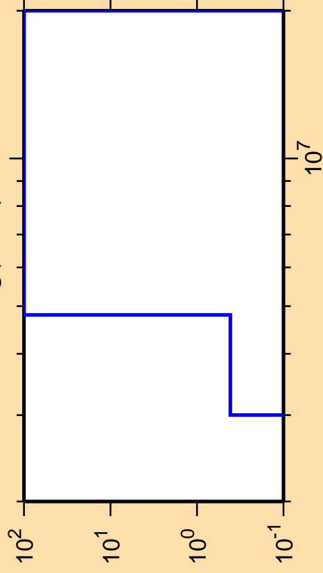
\Delta\sigma/\sigma vs. E for ^{193}\text{Hg}(n,n\alpha)
