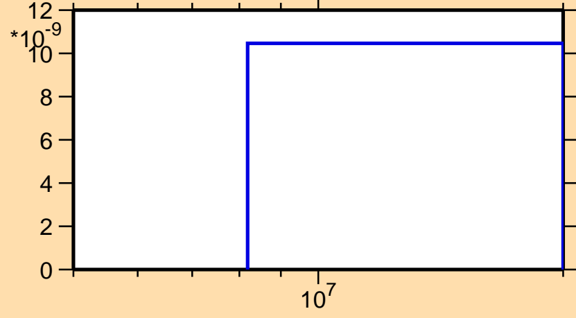
\sigma vs. E for ^{193}\text{Hg}(n,2n\alpha)
