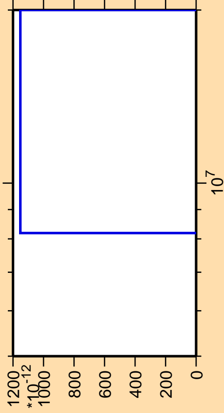
\Delta\sigma/\sigma vs. E for ^{193}\text{Hg}(\text{mt } 11)
