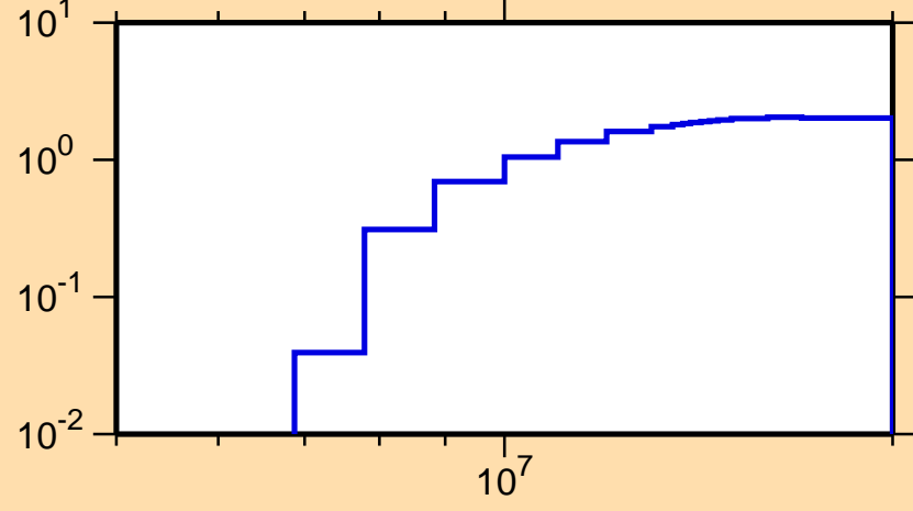
\sigma vs. E for ^{195}\text{Hg}(n,2n)
