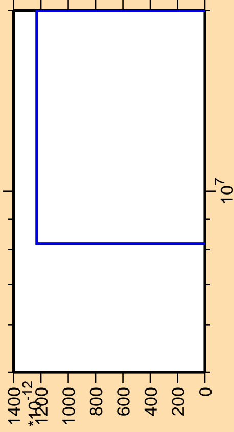
\Delta\sigma/\sigma vs. E for ^{195}\text{Hg}(\text{mt } 11)
