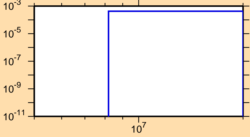
\sigma vs. E for ^{195}\text{Hg}(n,d)
