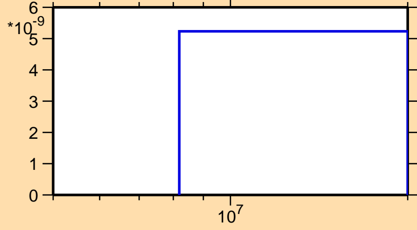
\sigma vs. E for ^{195}\text{Hg}(n,2n\alpha)
