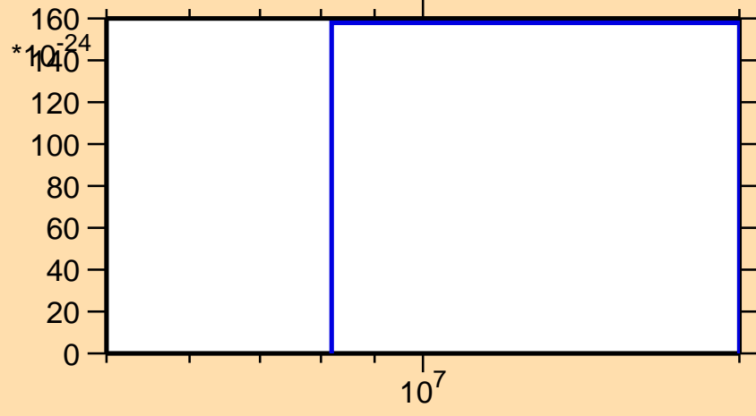
\sigma vs. E for ^{195}\text{Hg}(\text{mt } 11)
