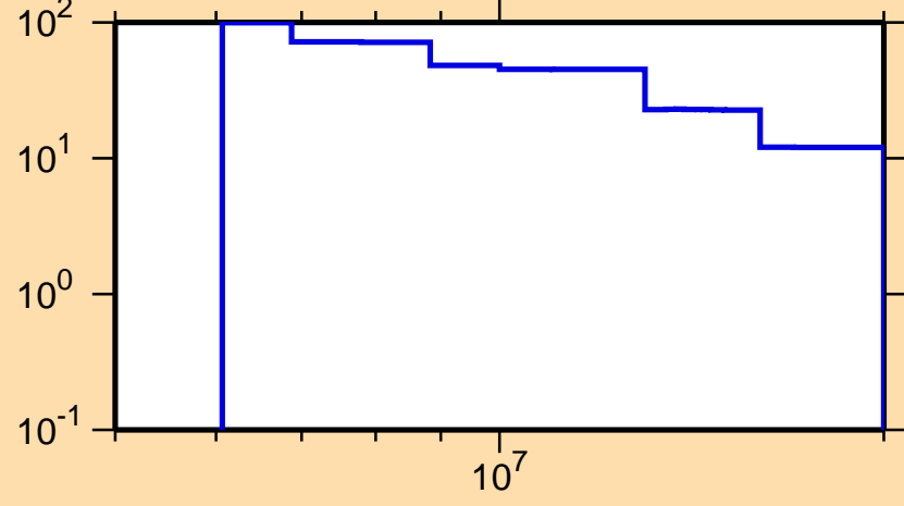
\Delta\sigma/\sigma vs. E for ^{195}\text{Hg}(n,2n)
