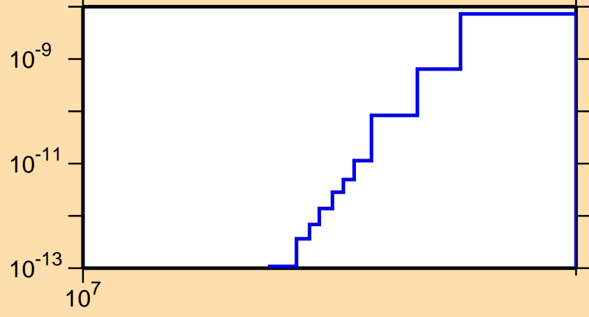
\sigma vs. E for ^{195}\text{Hg}(n,\text{He}3)
