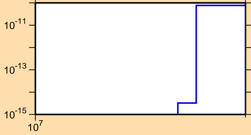
\sigma vs. E for ^{195}\text{Hg}(n,\text{nt})
