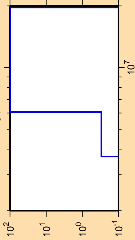
\Delta\sigma/\sigma vs. E for ^{195}\text{Hg}(n,n\alpha)
