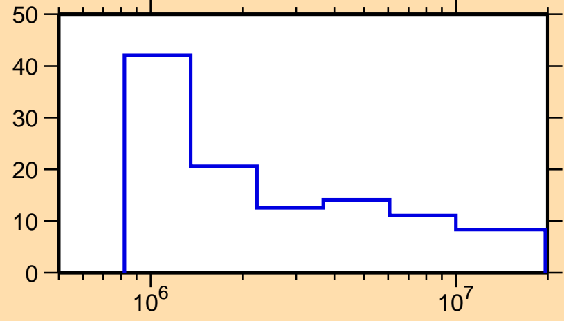
\Delta\sigma/\sigma vs. E for ^{195}\text{Hg}(n,n\text{onel.})
