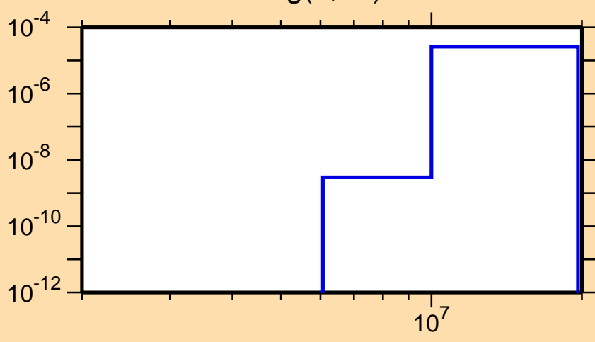
\sigma vs. E for ^{195}\text{Hg}(n,n\alpha)
