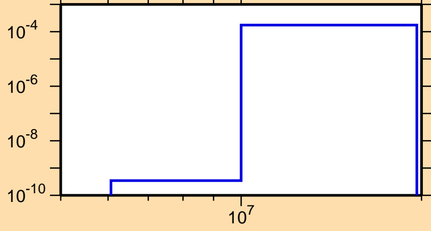
\sigma vs. E for ^{195}\text{Hg}(n,np)
