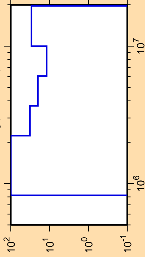
\Delta\sigma/\sigma vs. E for ^{195}\text{Hg}(n,\text{ncont.})
