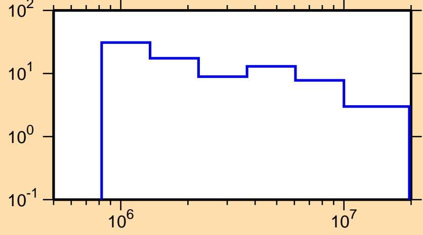
\Delta\sigma/\sigma vs. E for ^{195}\text{Hg}(n,\text{tot.})
