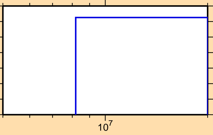
\sigma vs. E for ^{195}\text{Hg}(n,nt)
