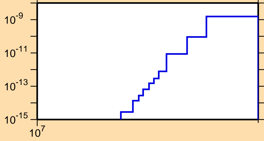
\sigma vs. E for ^{196}\text{Hg}(n,\text{He3})
