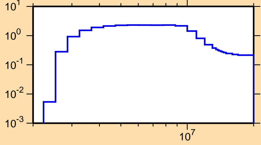
\sigma vs. E for ^{196}\text{Hg}(n,n\text{cont.})
