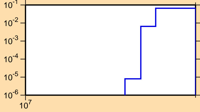
\sigma vs. E for ^{196}\text{Hg}(n,3n)
