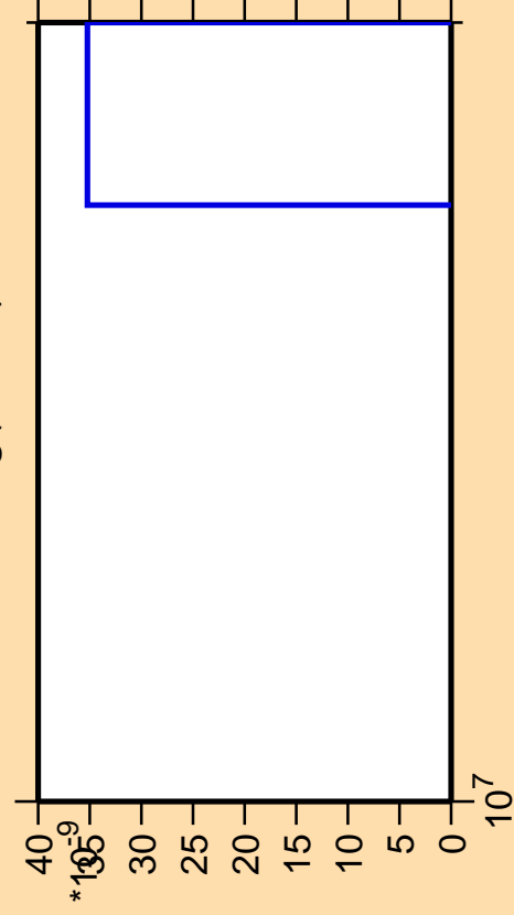
\Delta\sigma/\sigma vs. E for ^{196}\text{Hg}(\text{mt } 11)
