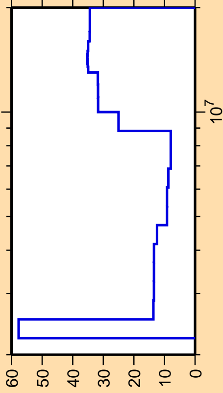
\Delta\sigma/\sigma vs. E for ^{196}\text{Hg}(n,\text{ncont.})
