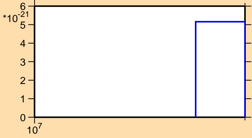
\sigma vs. E for ^{196}\text{Hg}(\text{mt } 11)
