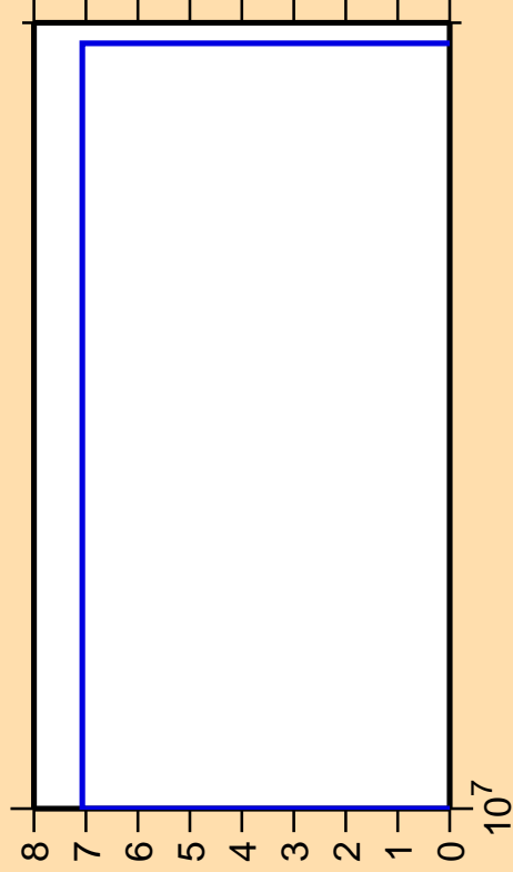
\Delta\sigma/\sigma vs. E for ^{196}\text{Hg}(n,nt)
