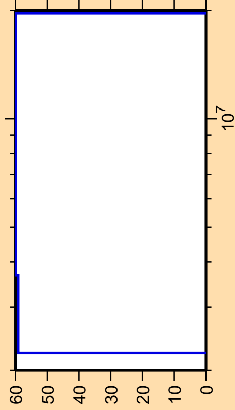
\Delta\sigma/\sigma vs. E for ^{196}\text{Hg}(n,\gamma)
