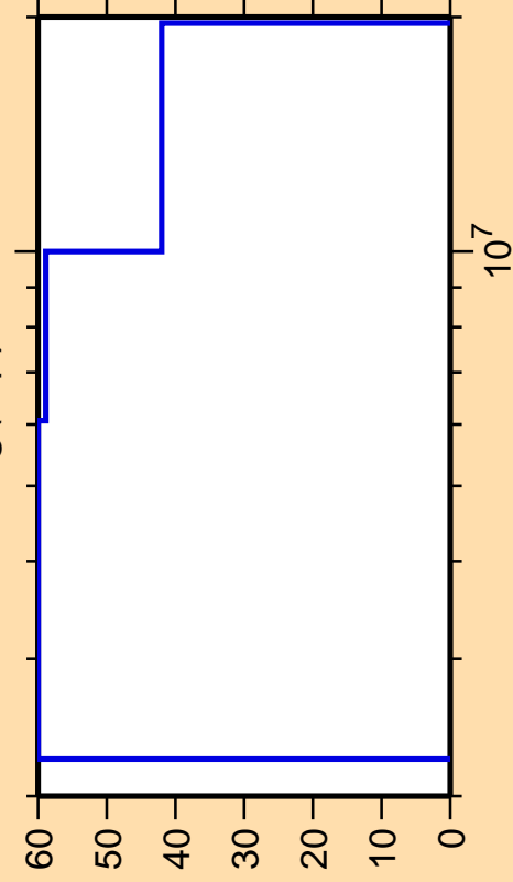
\Delta\sigma/\sigma vs. E for ^{196}\text{Hg}(n,p)
