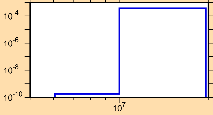
\sigma vs. E for ^{196}\text{Hg}(n,np)
