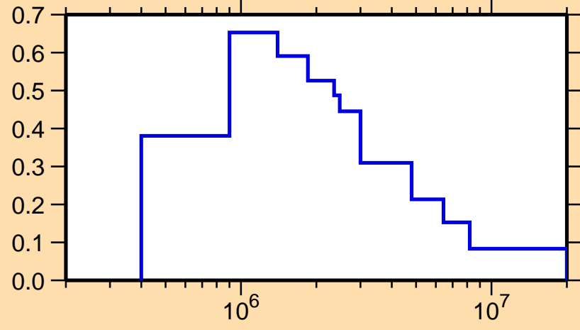
\sigma vs. E for ^{196}\text{Hg}(n,n_1)
