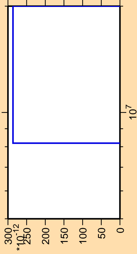
\Delta\sigma/\sigma vs. E for ^{196}\text{Hg}(\text{mt } 11)
