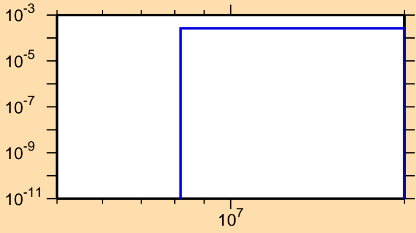
\sigma vs. E for ^{196}\text{Hg}(n,d)
