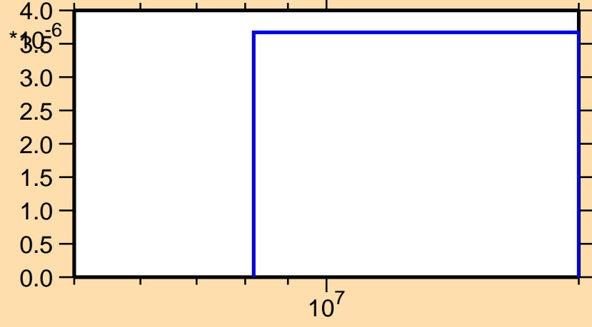
\sigma vs. E for ^{196}\text{Hg}(n,t)
