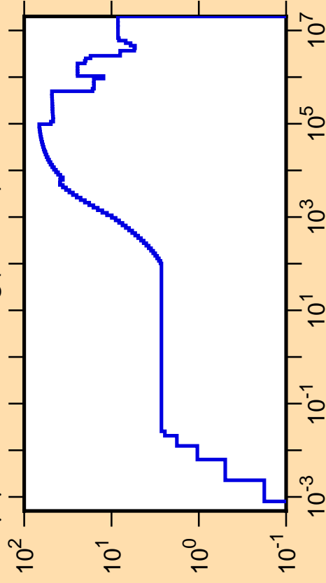
\Delta\mu/\mu vs. E for ^{197}\text{Hg}(\text{mt251})
