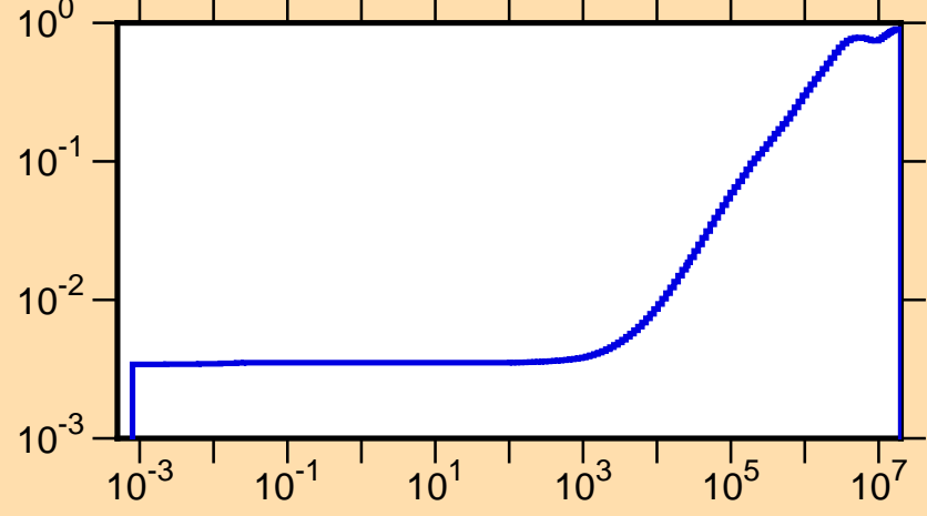
\mu vs. E for ^{197}\text{Hg}(\text{mt251})
