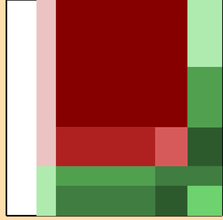
\Delta\sigma/\sigma vs. E for ^{197}\text{Hg}(n,2n)
