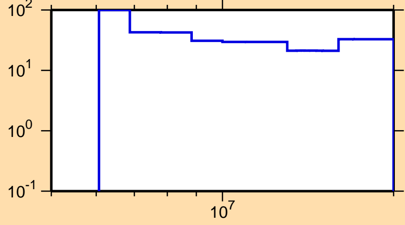
\Delta\sigma/\sigma vs. E for ^{197}\text{Hg}(n,2n)
