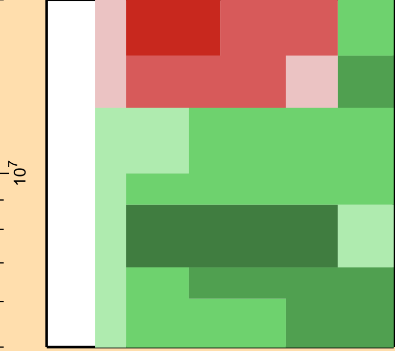
\Delta\sigma/\sigma vs. E for ^{197}\text{Hg}(n,2n)
