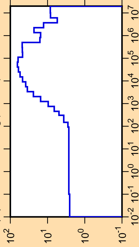
\Delta\mu/\mu vs. E for ^{197}\text{Hg}(\text{mt251})
