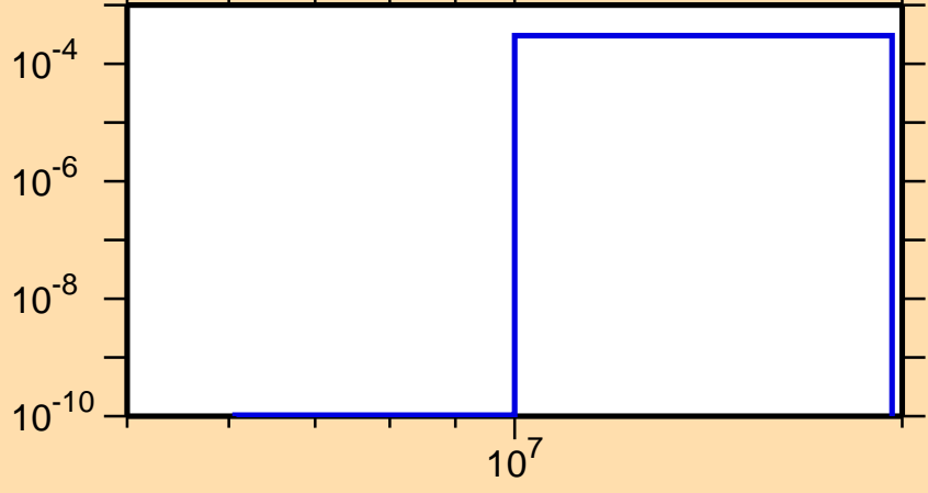
\sigma vs. E for ^{197}\text{Hg}(n,d)
