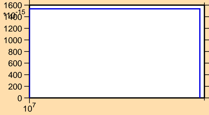
\sigma vs. E for ^{197}\text{Hg}(n,\text{nt})
