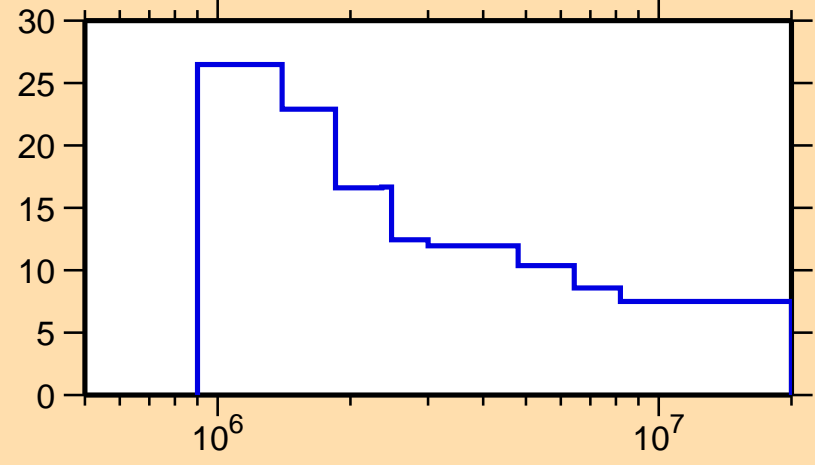
\Delta\sigma/\sigma vs. E for ^{197}\text{Hg}(n,n\text{onel.})
