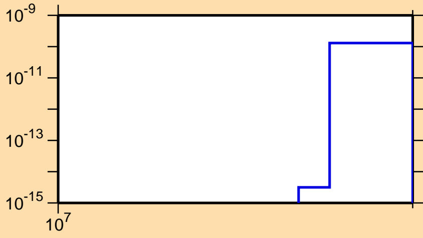
\sigma vs. E for ^{197}\text{Hg}(n,nt)
