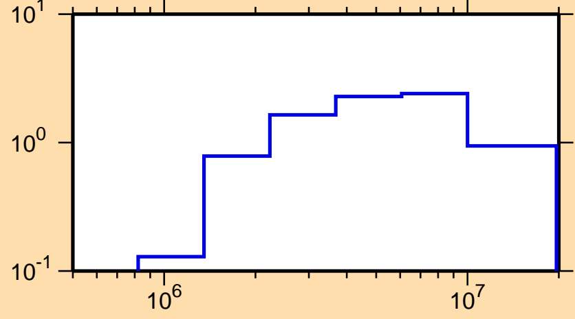
\sigma vs. E for ^{197}\text{Hg}(n,n\text{cont.})
