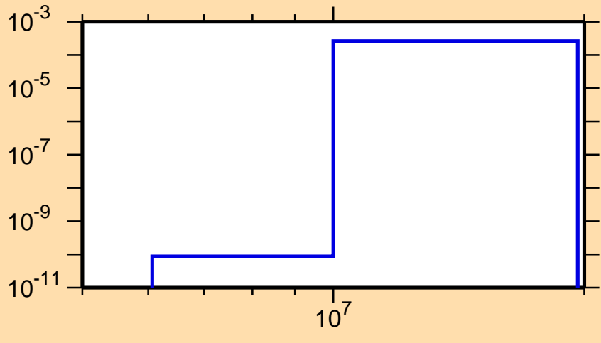
\sigma vs. E for ^{197}\text{Hg}(n,d)
