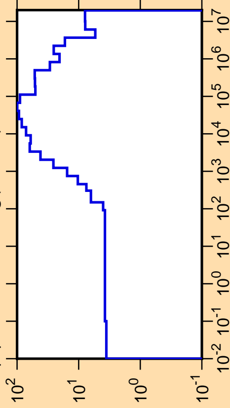
\Delta\mu/\mu vs. E for ^{198}\text{Hg}(\text{mt251})
