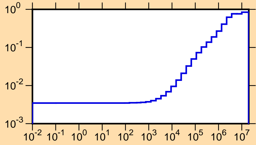
\mu vs. E for ^{198}\text{Hg}(\text{mt251})
