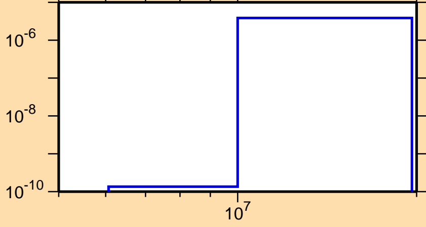
\sigma vs. E for ^{198}\text{Hg}(n,n\alpha)
