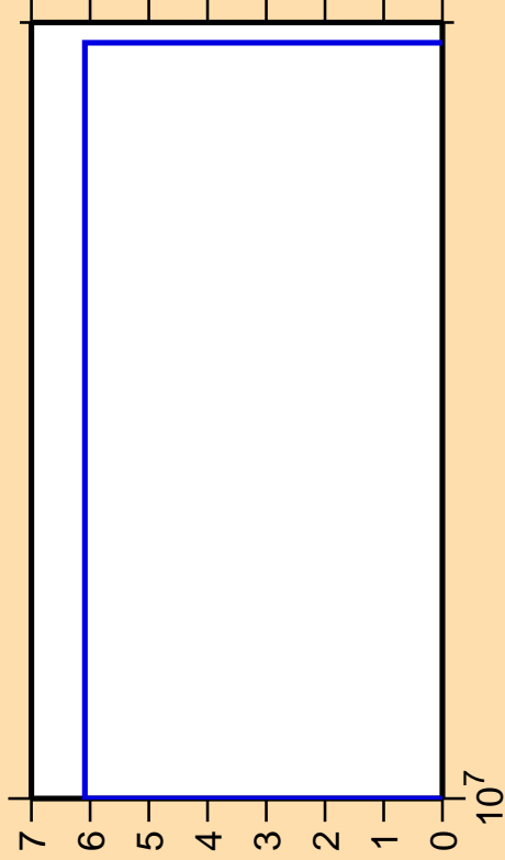
\Delta\sigma/\sigma vs. E for ^{198}\text{Hg}(n,\text{nt})
