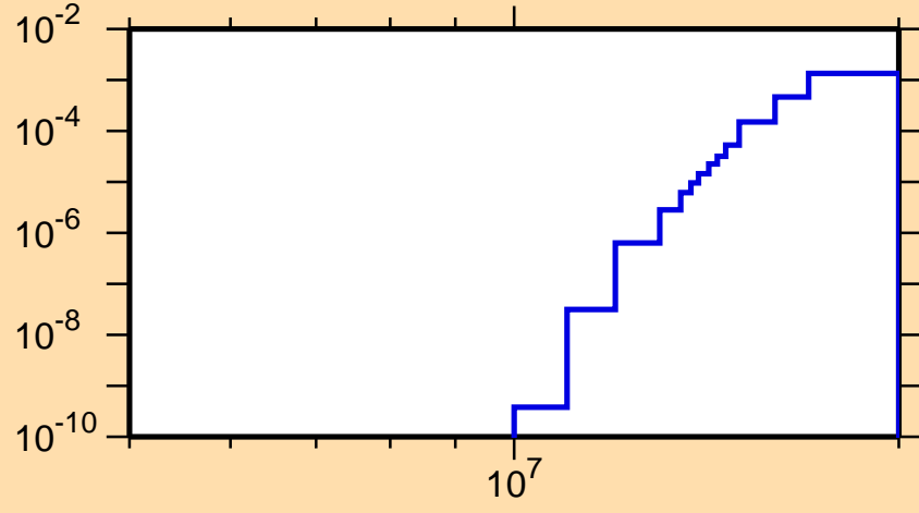
\sigma vs. E for ^{199}\text{Hg}(n,np)
