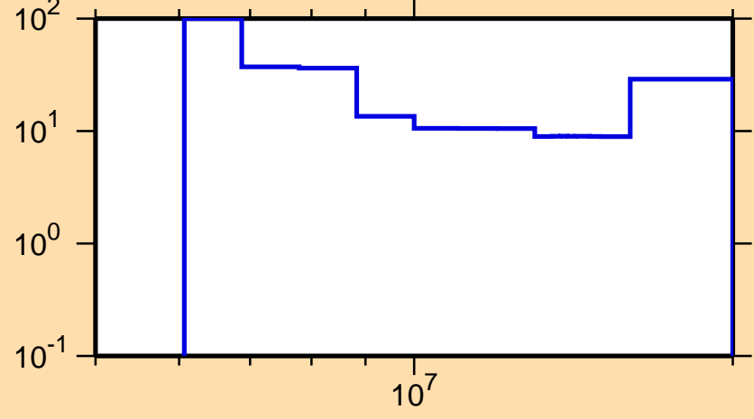
\Delta\sigma/\sigma vs. E for ^{199}\text{Hg}(n,2n)
