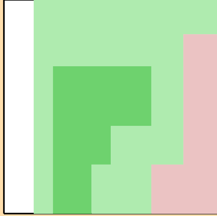
\Delta\sigma/\sigma vs. E for ^{199}\text{Hg}(n,2n)
