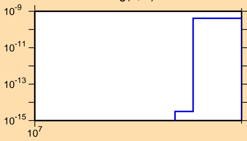
\sigma vs. E for ^{199}\text{Hg}(n,nt)
