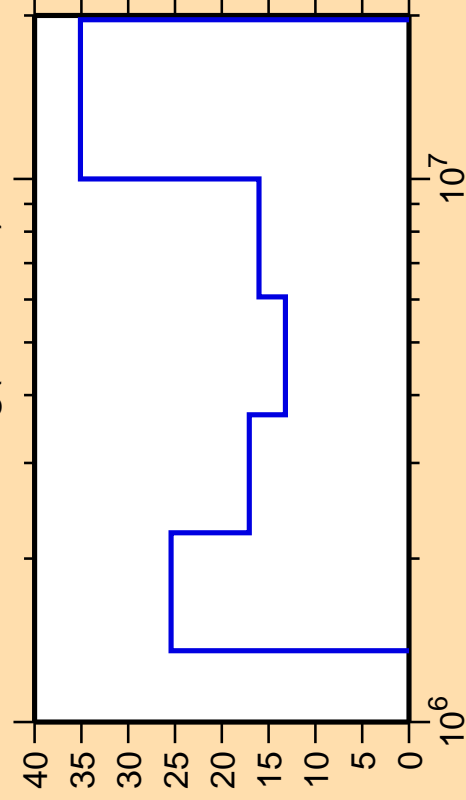
\Delta\sigma/\sigma vs. E for ^{199}\text{Hg}(n,\text{ncont.})
