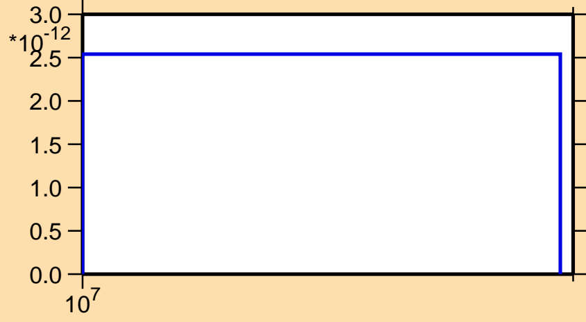
\sigma vs. E for ^{199}\text{Hg}(n,\text{nt})
