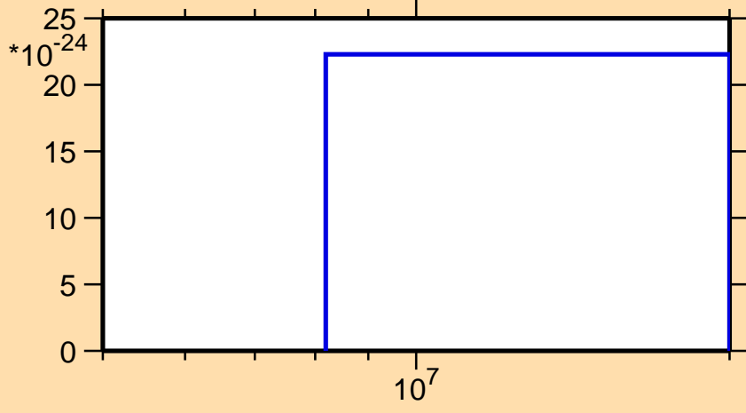
\sigma vs. E for ^{199}\text{Hg}(\text{mt } 11)
