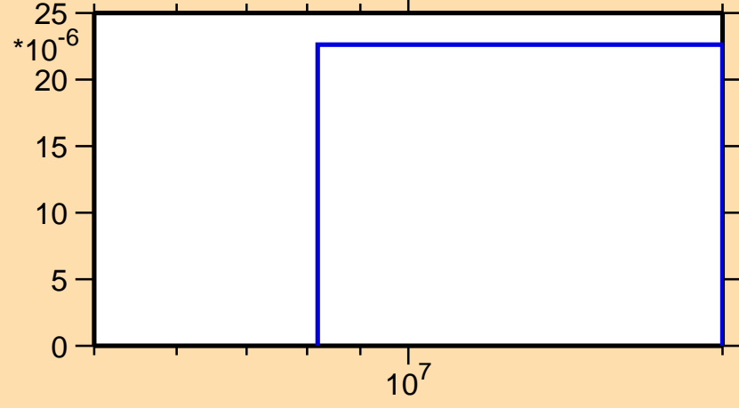
\sigma vs. E for ^{199}\text{Hg}(n,t)
