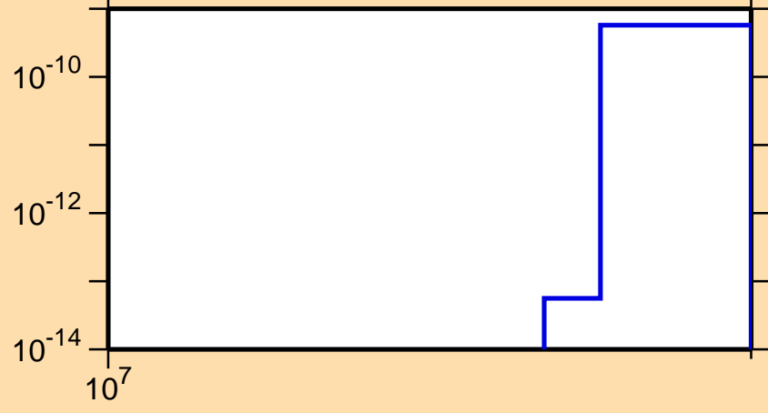
\sigma vs. E for ^{199}\text{Hg}(n,nt)
