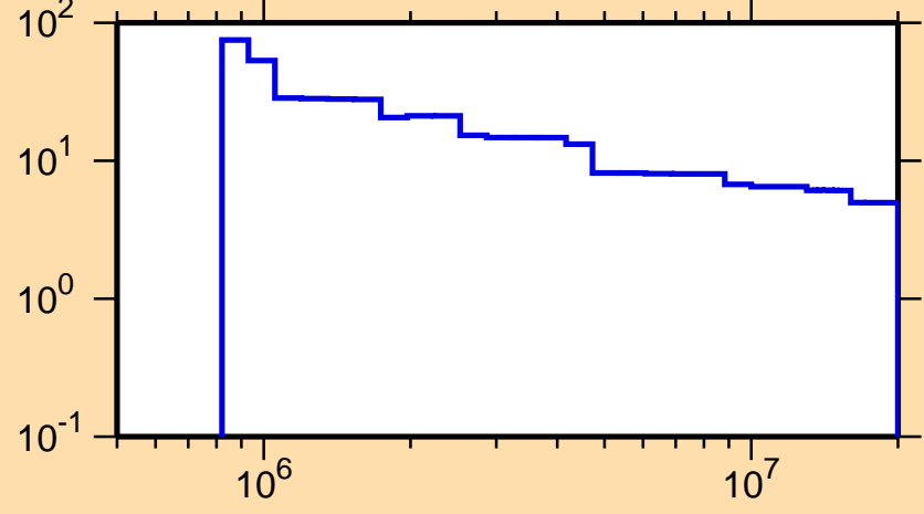
\Delta\sigma/\sigma vs. E for ^{199}\text{Hg}(n,n\text{onel.})
