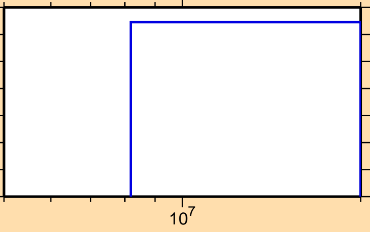
\sigma vs. E for ^{199}\text{Hg}(n,\text{nd})
