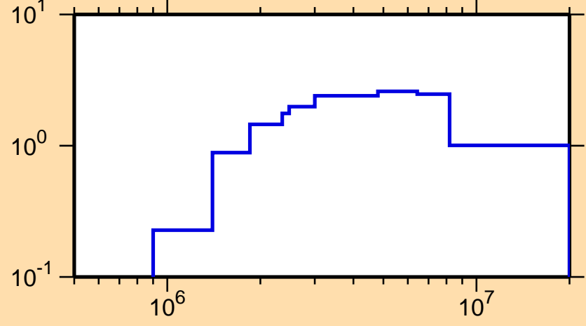
\sigma vs. E for ^{199}\text{Hg}(n,n\text{cont.})
