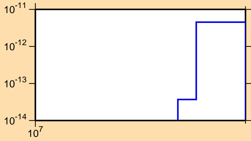
\sigma vs. E for ^{200}\text{Hg}(n,\text{He}3)
