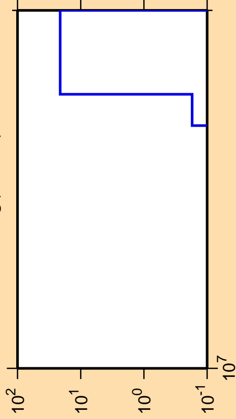
\Delta\sigma/\sigma vs. E for ^{200}\text{Hg}(n,\text{He}3)
