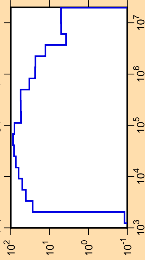
\Delta\mu/\mu vs. E for ^{200}\text{Hg}(\text{mt251})
