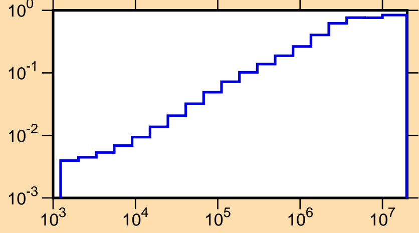
\mu vs. E for ^{200}\text{Hg}(\text{mt251})
