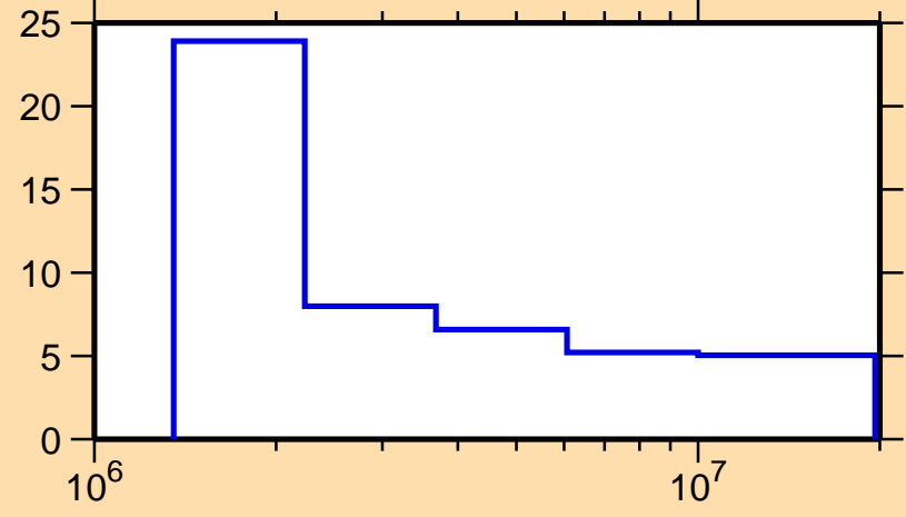
\Delta\sigma/\sigma vs. E for ^{200}\text{Hg}(n,n\text{onel.})
