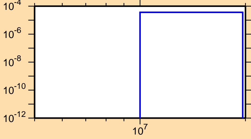
\sigma vs. E for ^{200}\text{Hg}(n,np)
