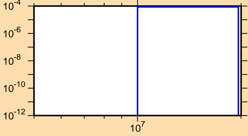
\sigma vs. E for ^{200}\text{Hg}(n,d)
